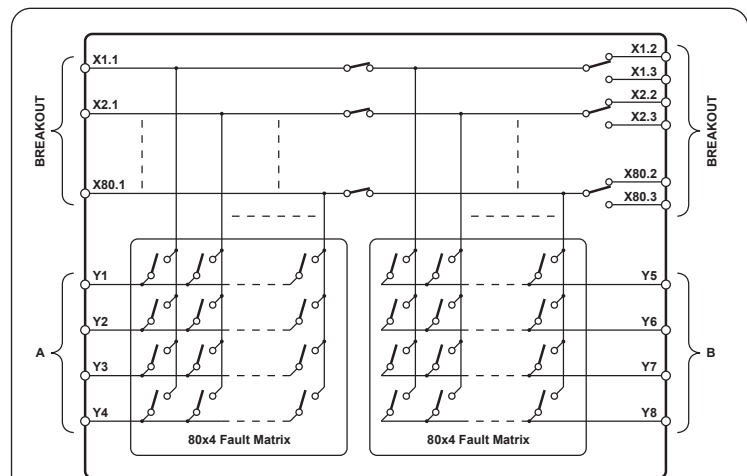
Schematic of the 40-592A-104 Dual 80x4 FIBO High Density Matrix Module with 3-pin breakout (switches are shown in their default state)
