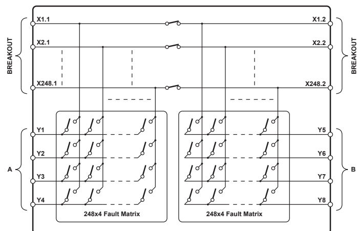
Schematic of the 40-592A-118 Dual 248x8 FIBO High Density FIBO Matrix Module with 2-pin breakout (switches are shown in their default state)
