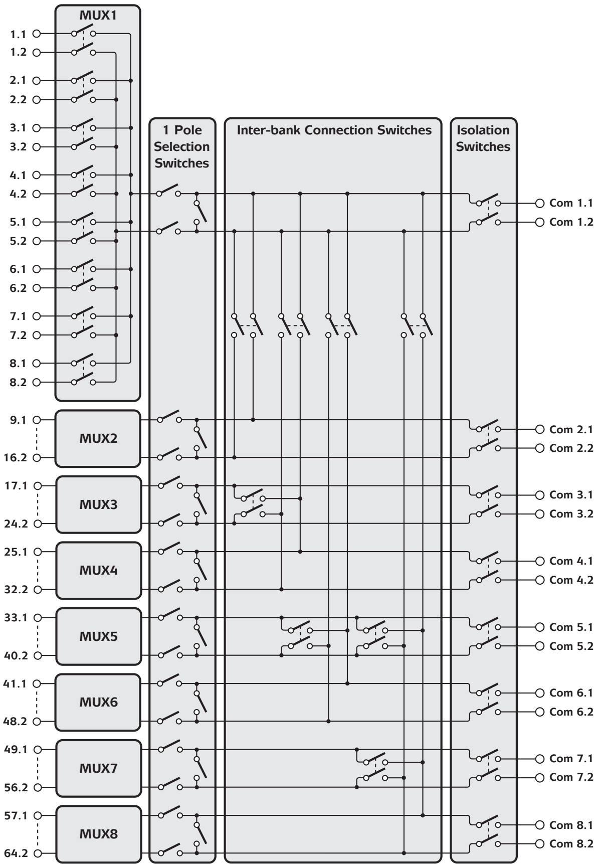
Functional Diagram of 40-681 Solid State Versatile Multiplexer
