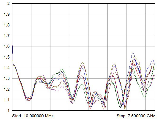
VSWR Channel to COM for 40-883-001 showing all paths up to 7.5 GHz
