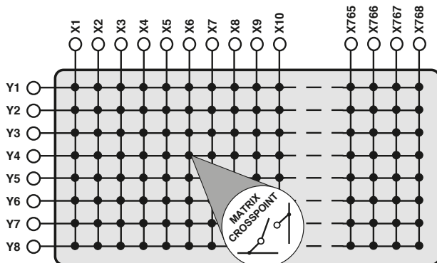
Simplified Diagram For 65-223 Configured as a 768x8 Matrix
