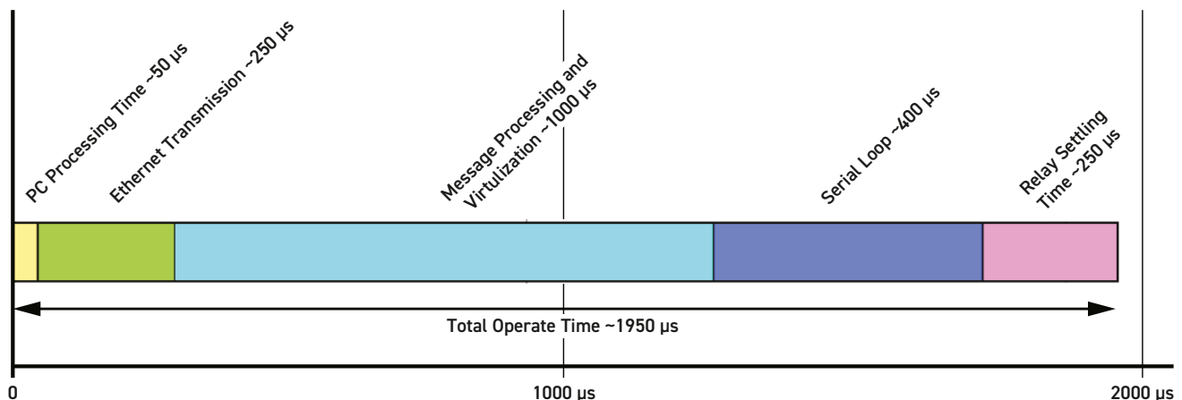
Speed of Operation Diagram For The 65-223
