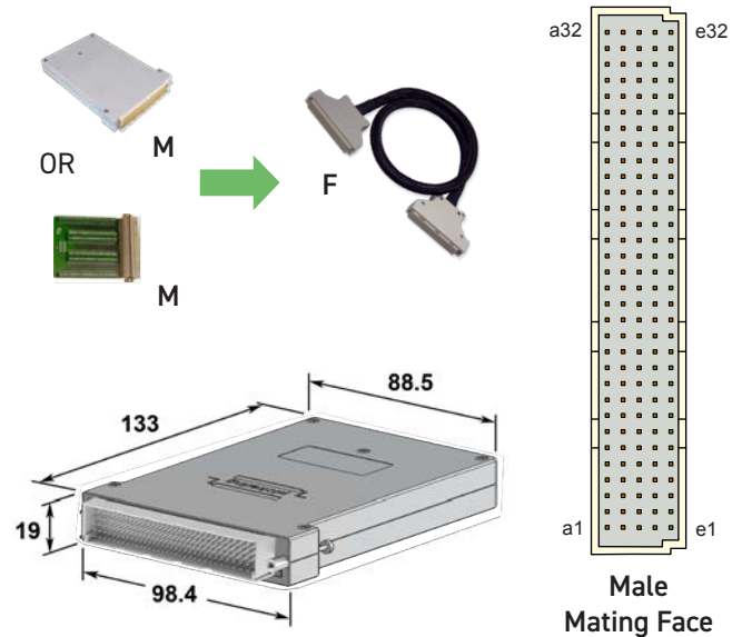
Connector Block Dimensions
