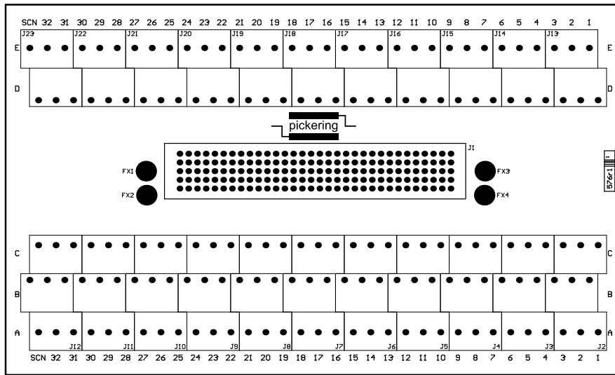
PCB Layout
