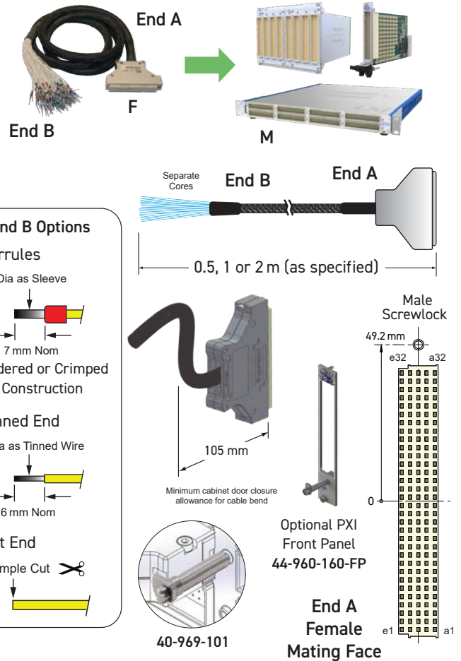
160-Pin DIN41612 Cable Assy - Female to Unterminated
