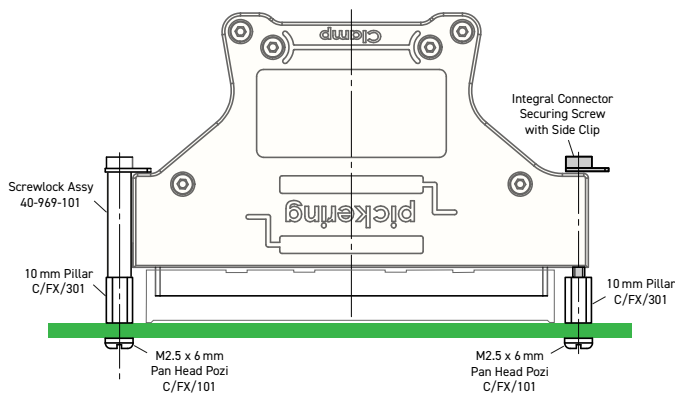
Additional Fixings that May be Required to Secure a Mating Connector
